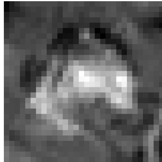
Feature Map 4
