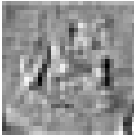
Feature Map 3
