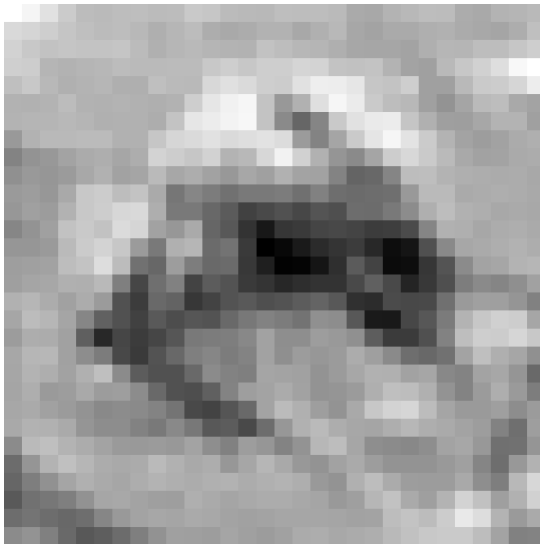
Feature Map 2
