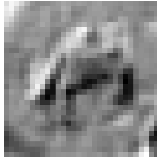
Feature Map 8
