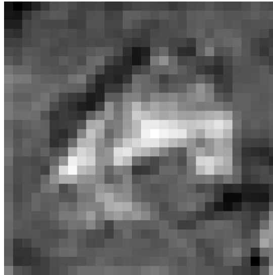
Feature Map 7
