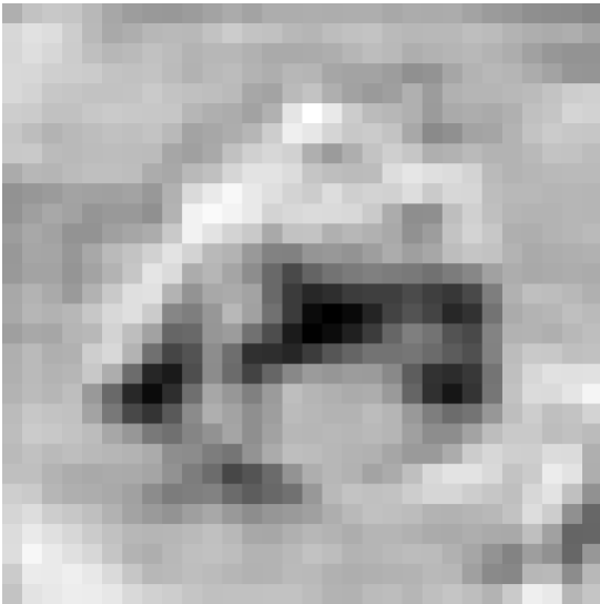
Feature Map 5
