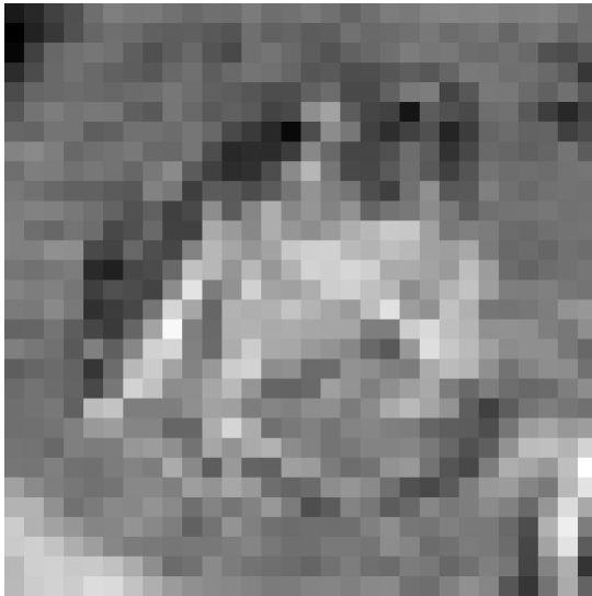
Feature Map 6
