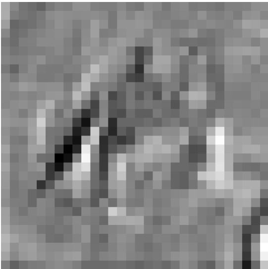
Feature Map 1
